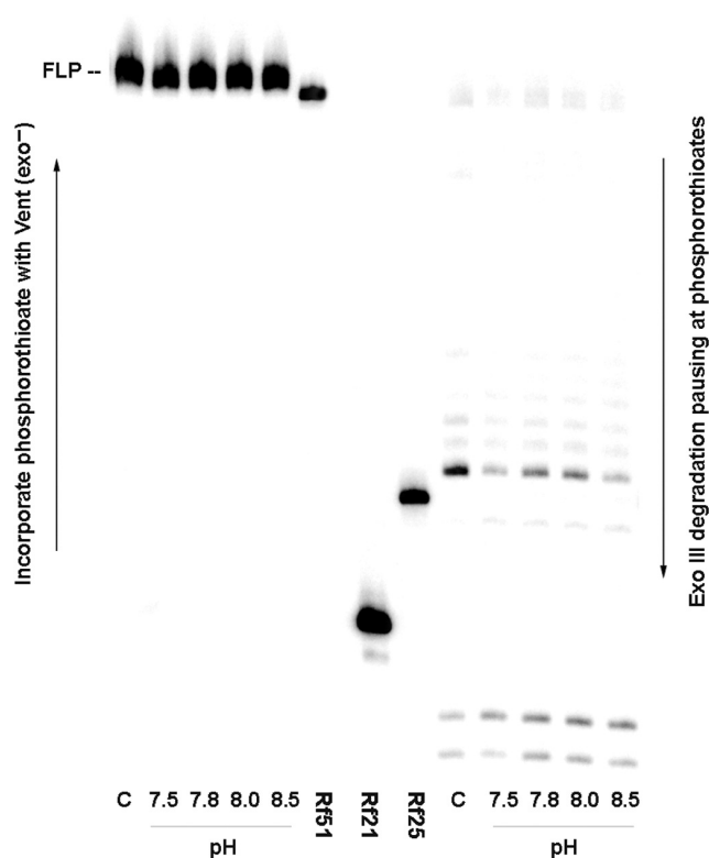
Figure 5. Retention of the \text{dZ}:\text{dP} pair in products generated by 16.6 theoretical PCR cycles (using Taq ) as a function of pH. Left: Seven cycles of ‘analytical primer extension’ by Vent ( \text{exo}^- ) with \text{dZTP}\alpha\text{S} , \text{dP}\alpha\text{S} and \text{dNTPs} converts 5' - ^{32}\text{P} labeled primer (P-RS-S16) to FLP with a phosphorothioate linkage joining nucleotides 25 and 26 (arising via incorporation of \text{dZTP}\alpha\text{S} opposite retained \text{dP} in the amplicon) at pH 8.5. Right: Digestion of FLP using Exo III (20 U, final concentration 0.5 U/ \mu\text{l} ), giving pause bands where a phosphorothioate linker is present, either from \text{dZTP}\alpha\text{S} incorporation (expected between nucleotides 25 and 26) or from the synthetic primer (between nucleotides 16 and 17). Control (C) used synthetic templates (containing 100% \text{dZ}:\text{dP} pair at position 26). Lanes Rf51, Rf21 and Rf25 hold reference 51-, 21- and 25-mers. Noticeably stronger are Exo III digestion bands indicating greater retention of \text{dZ}:\text{dP} pair at pH 7.8 and 8.0 than at 7.5 or 8.5.
